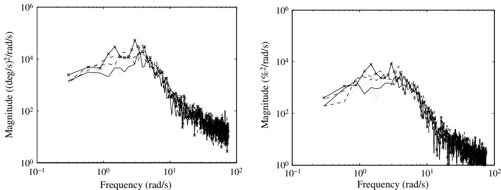
Fig. 12 Power spectral density in inverted configuration: a) roll rate, and b) aileron deflection. Smaller tail: dashed line, small tail: dotted-dashed line, normal tail: line, big tail: dotted line, bigger tail: dashed line with x.
