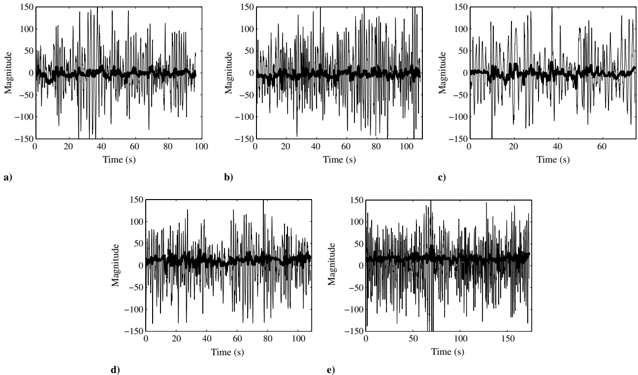
Fig. 7 Time Responses in upright configuration: a) smaller tail, b) small tail, c) normal tail, d) big tail, and e) bigger tail, where the roll rate is denoted with a thin line and the aileron deflection is denoted with a thick line.
