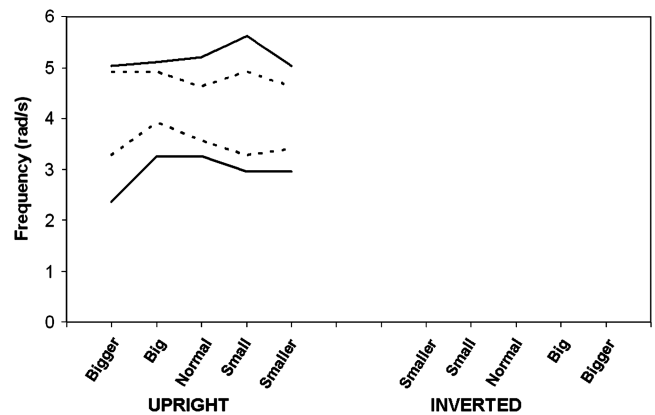
Fig. 16 Upper and lower bounds of uncommanded wing rock frequency from PSDs (line) and wavelets (dotted line).
