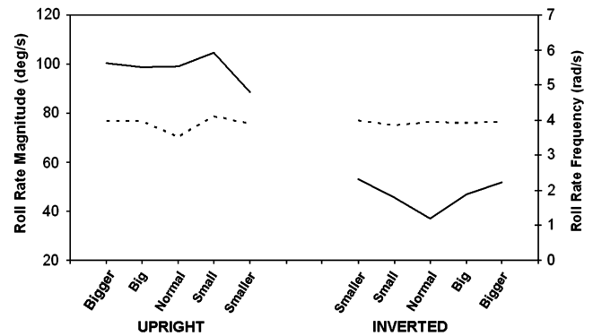
Fig. 15 Mean roll rate peak magnitudes (line) and peak-to-peak frequencies (dotted line).
