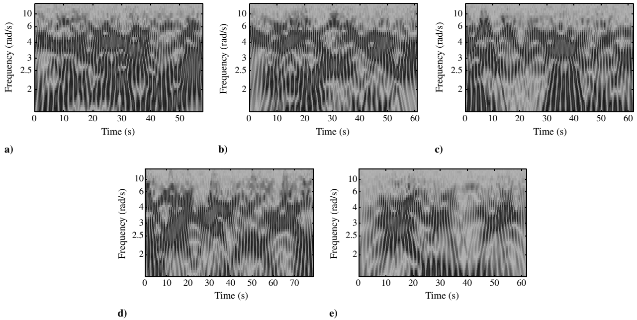
Fig. 13 Wavelet transforms of roll rate in inverted configuration: a) smaller tail, b) small tail, c) normal tail, d) big tail, and e) bigger tail.
