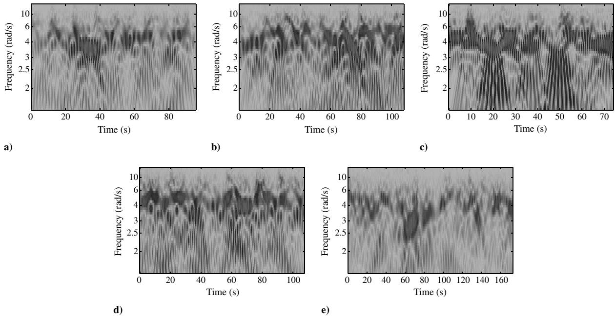
Fig. 9 Wavelet transforms of roll rate in upright configuration: a) smaller tail, b) small tail, c) normal tail, d) big tail, and e) bigger tail.
