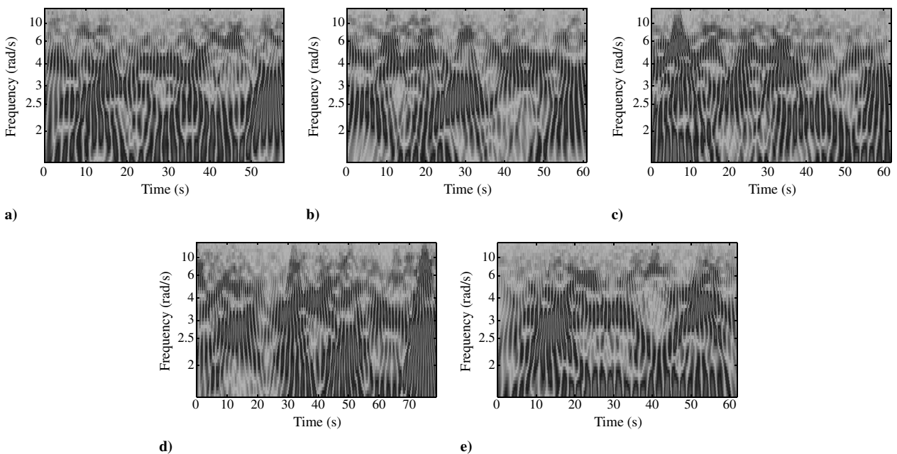
Fig. 14 Wavelet transforms of aileron deflection in inverted configuration: a) smaller tail, b) small tail, c) normal tail, d) big tail, and e) bigger tail.
