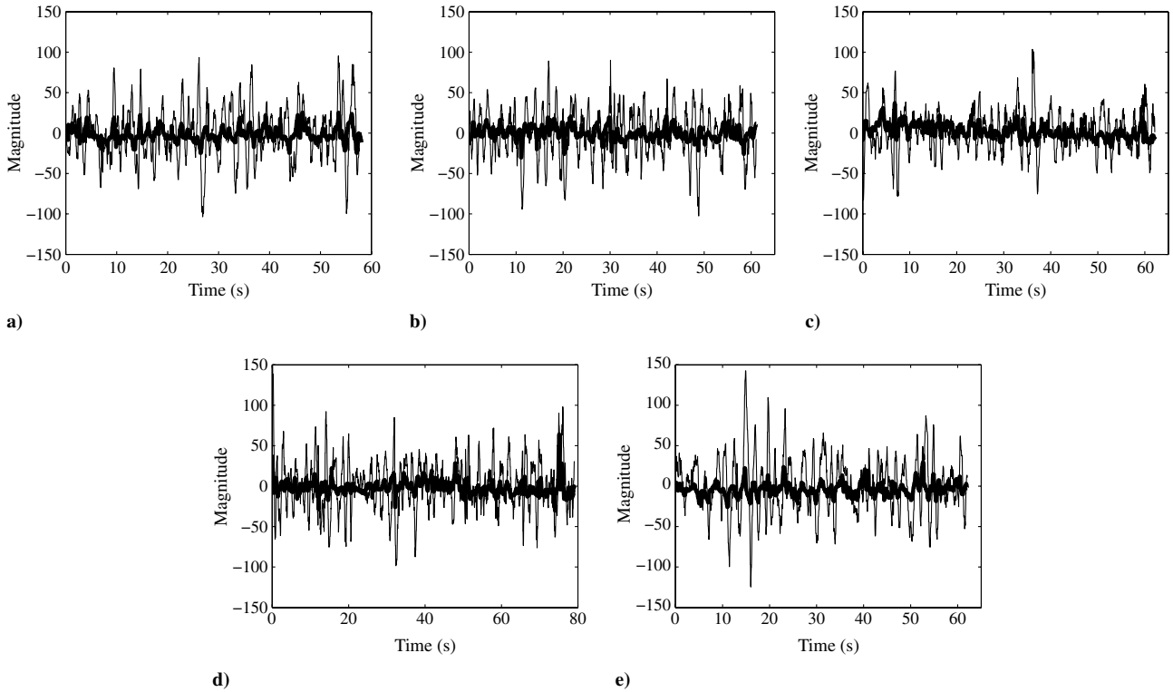
Fig. 11 Time responses in inverted configuration: a) smaller tail, b) small tail, c) normal tail, d) big tail, and e) bigger tail, where the roll rate is denoted with a thin line and the aileron deflection is denoted with a thick line.
