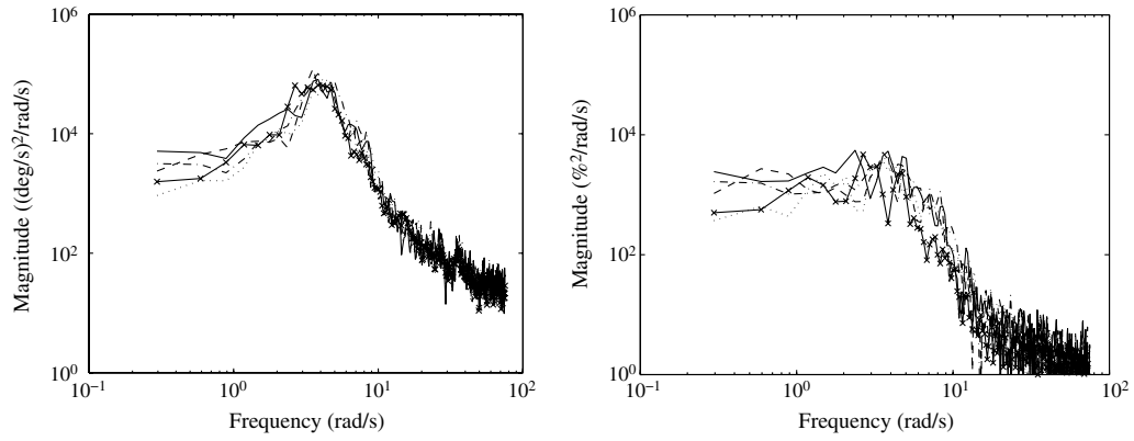
Fig. 8 Power spectral density in upright configuration: a) roll rate, and b) aileron deflection. Smaller tail: dashed line, small tail: dotted-dashed line, normal tail: line, big tail: dotted line, bigger tail: dashed line with x.
