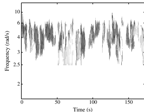
Fig. 17 Filtered wavelet transform of roll rate with upright bigger tail.
