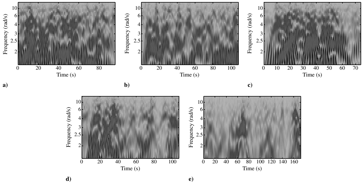
Fig. 10 Wavelet transforms of aileron deflection in upright configuration: a) smaller tail, b) small tail, c) normal tail, d) big tail, and e) bigger tail.
