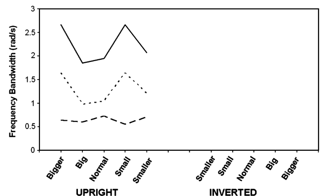
Fig. 18 Average uncommanded wing rock bandwidth: bounds from PSDs (line) and wavelets (dotted line), and localized from wavelets (dashed line).
